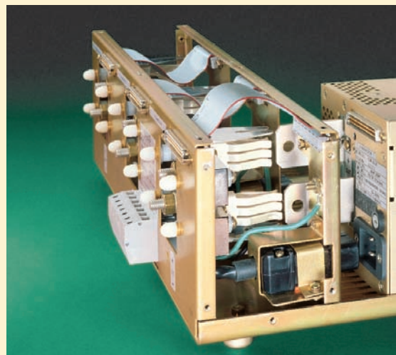
Rear view, cover removed, of the rack housing showing the heavy-duty bus-bar connections that make HSP's "Hot Swap" practical
