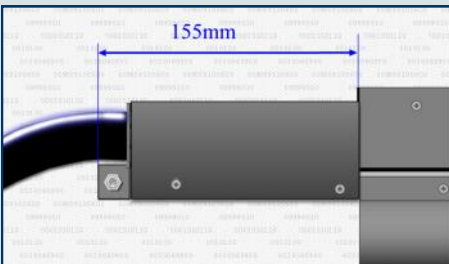
Dimension of terminals when using protective cover
