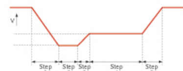
Voltage fluctuation test pattern
